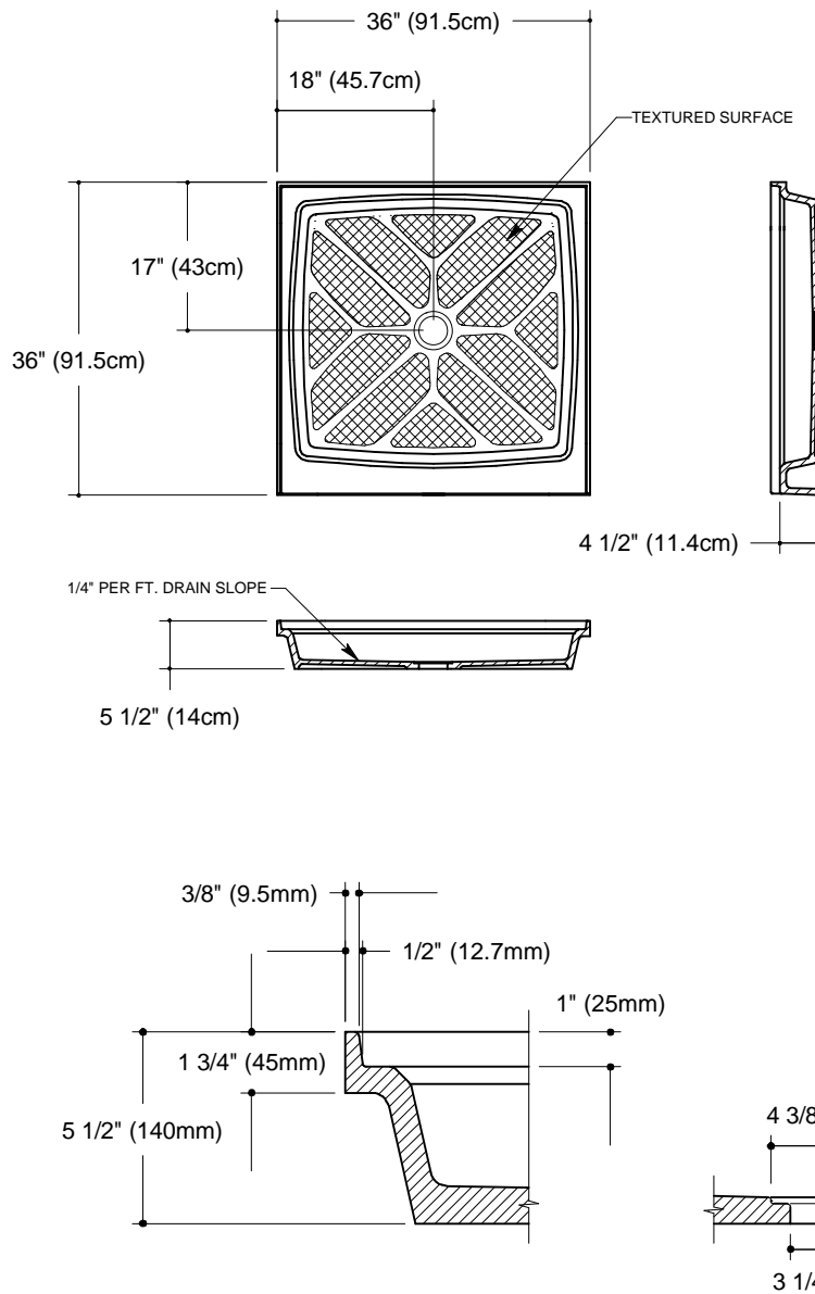
Sections showing water dam and drain details. (Lightweight option not shown)
