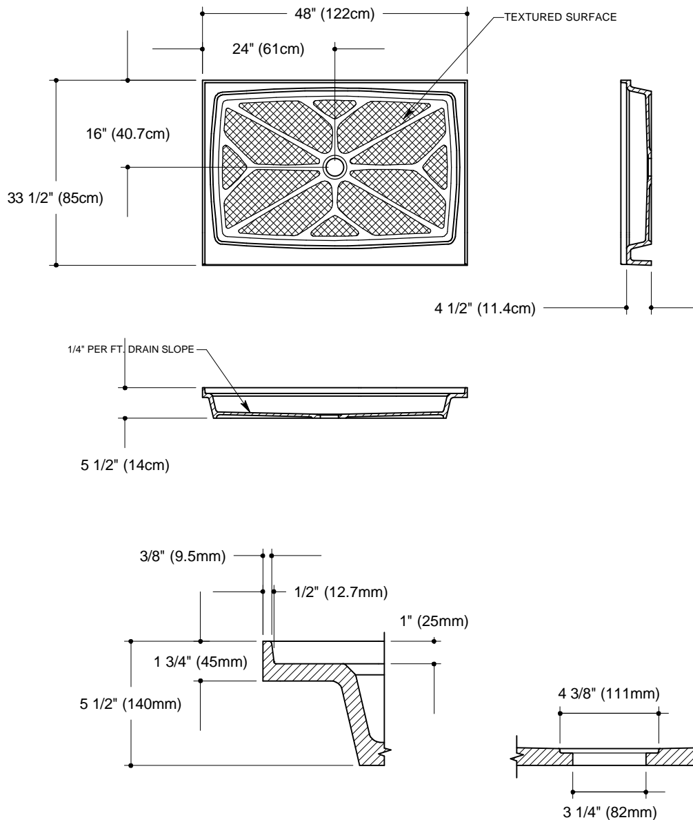
Sections showing water dam and drain details.
